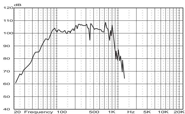
FREQUENCY RESPONSE (1W/1m)
